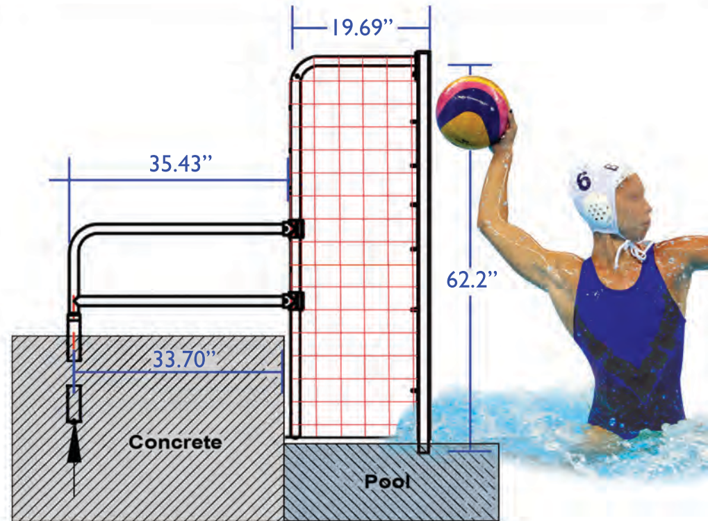
AW0616 UNIVERSAL WALL GOAL, LONG (SHALLOW WATER)
